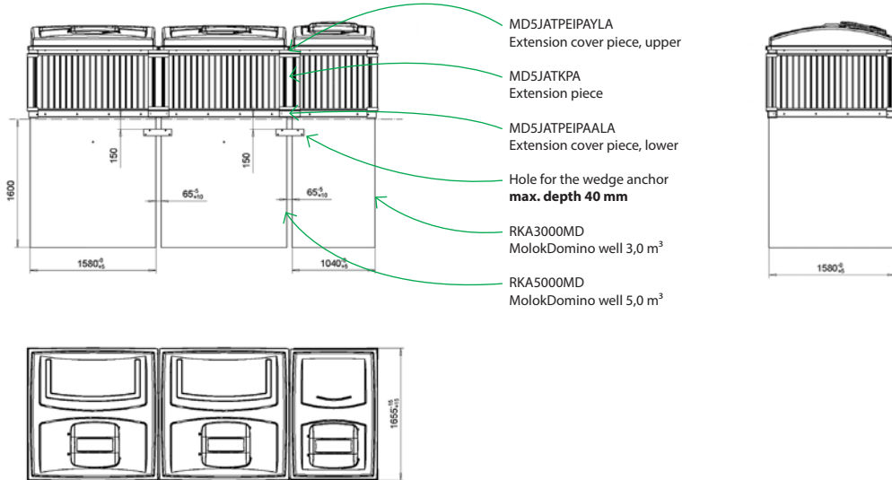
Figure 3. Example: installation of a group of three container bodies ( 5\text{m}^3 + 5\text{m}^3 + 3\text{m}^3 ) on level ground. Be sure to attach the extension pieces of the framing as well as the extension cover pieces at the installation site.
