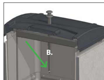
Figure 15. When the lid is placed on the container, the lifting beam (B) is installed, and secured with a M16x80 bolt + M16 nut.
