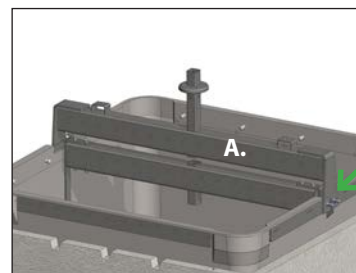
Figure 14. Upper beam (A) is fastened with 2 bolts at both ends.
