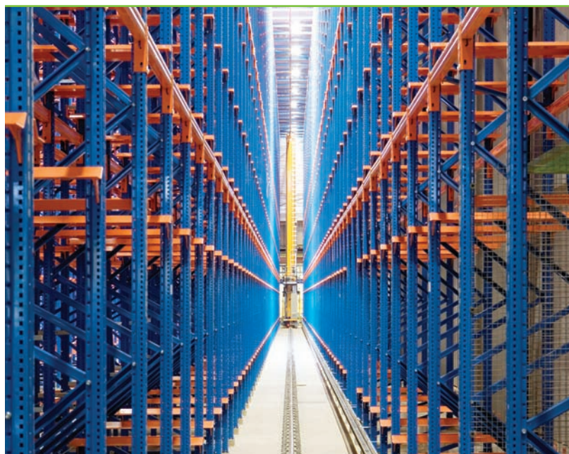
AS/RS application
